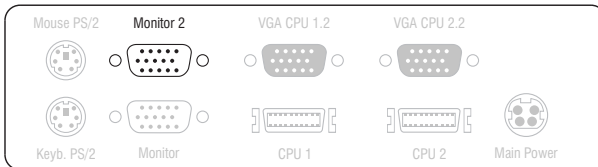
Figure 3: Interfaces to connect the second console monitor
